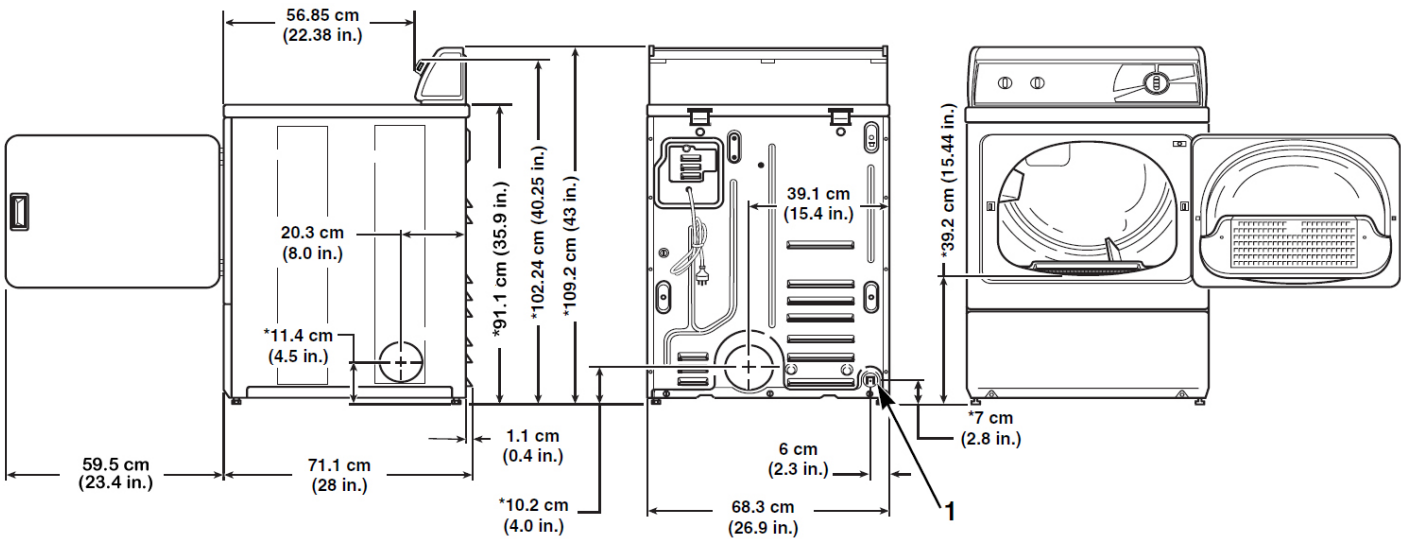
GAS DRYERS
